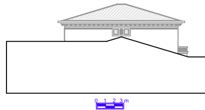
Elevation 03
